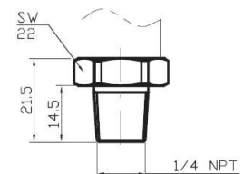
¼ NPT
